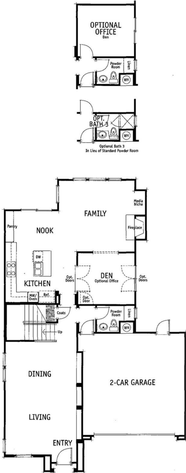
FIRST FLOOR
